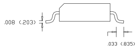
END VIEW
